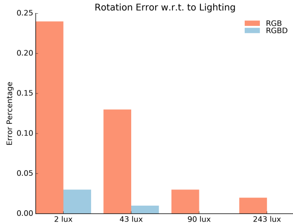
Fig. 12: Illumination vs. Error Percentage (0.1 = 10%). Data are captured at 65 cm away from the camera at a 40 degree angle.
