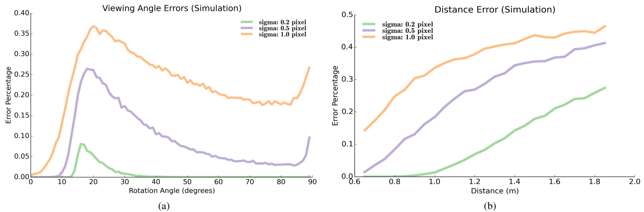
Fig. 5: Simulation results of Apriltag pose estimation under different noise level. In both simulations, four corners are projected onto a rendered image with some noise then computed their poses in each trail. In 5a, corners are projected to the center of the camera 0.8 meters away and rotated from 0^\circ to 90^\circ at 1^\circ interval. In 5b, the corners are projected at 40^\circ and moved from 0.6 meters to 1.8 meters at 0.1 meter interval. We sampled the poses from 10,000 trials for each experiment and computed the percentage of unacceptable poses base on a threshold.
