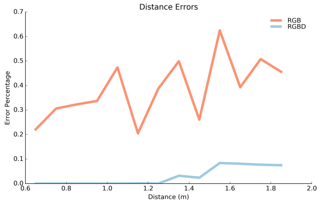
Fig. 10: Distance vs. Error Percentage (0.1 = 10%). Data are captured at a 10 cm increment from 65 cm to 185 cm.
