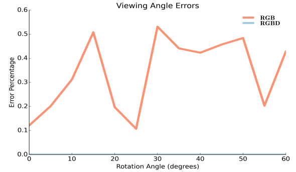
Fig. 9: Viewing Angle vs Error Percentage (0.1 = 10%) under different simulated noise level. The new RGBD based algorithm can resist noise in the RGB image and it vastly outperforms the original algorithm.
