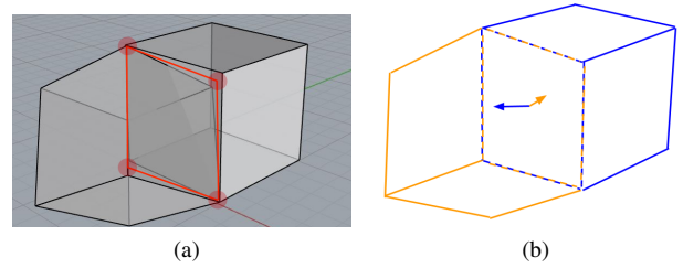
Fig. 4: The ambiguity effect can be demonstrated with two rendered cubes in the perspective view. The two cubes are rotated such that two faces are interlaced. The red square in 4a is a simulated projection of a square tag. The red circular regions denote the region of potential corner detection in a noisy scene. 4b is a sketch of the potential resulting 2D projection. The pose can converge to either one of the two faces.
