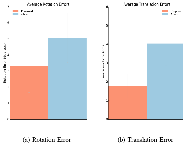
Fig. 13: Average pose errors compared with ar_track_alvar package.
